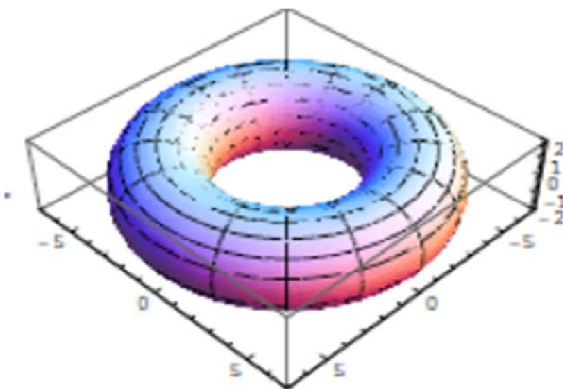
Two-dimensional torus
