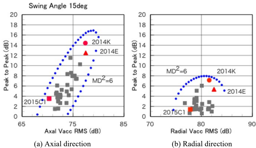
Fig.10 Threshold of visualized MD (Swing angle 15^\circ )
