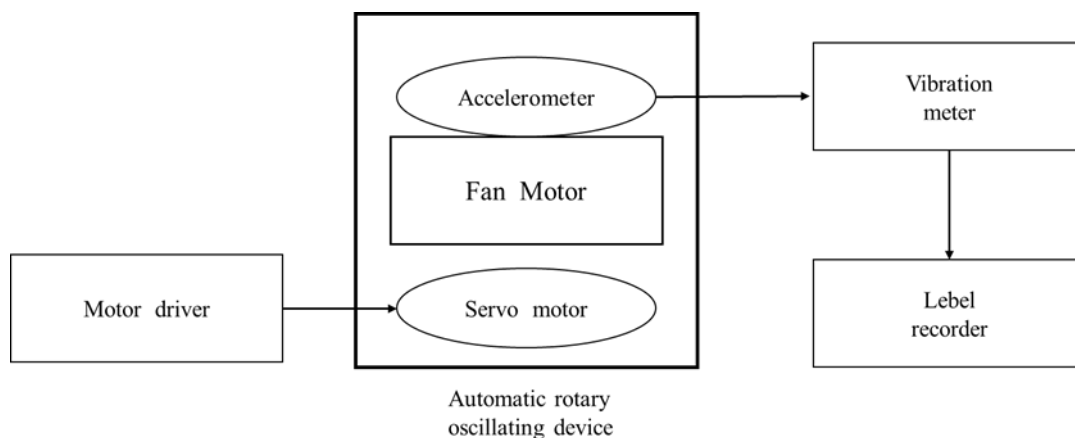
Fig.4 Block diagram of measurement system
