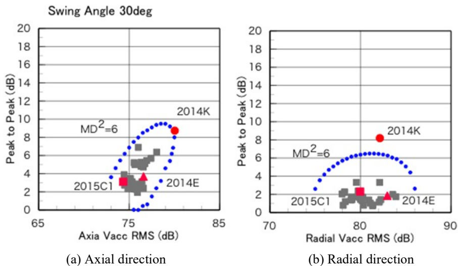
Fig.11 Threshold of visualized MD (Swing angle 30^\circ )
